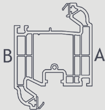
705545 95mm Z Mullion
