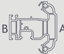
703538 Internally Beaded Sash
