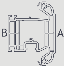
705543 95mm T Mullion
