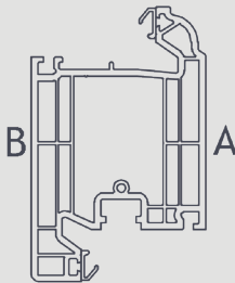
705540 Door Sash Open In
